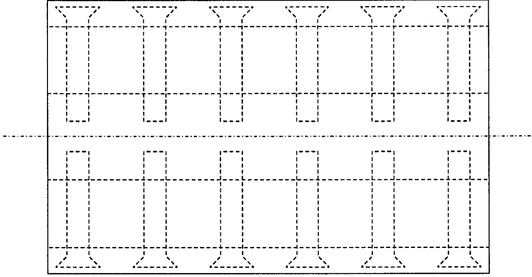
Figure 5.5: 7.5kW axially-laminated rotor axial view.
