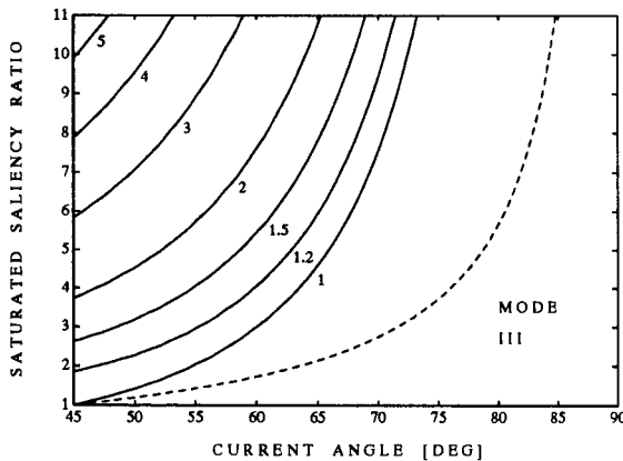
Figure 6: CPSR for constant saturation model.
