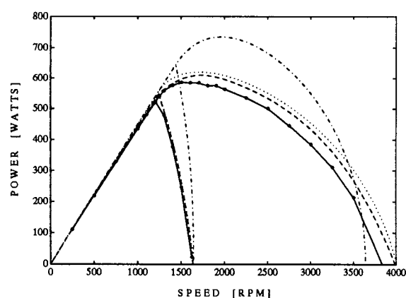
Figure 11: 2kW SPM torque and power versus speed results with and without field-weakening when operated at reduced voltage. Measured results (solid line), lossless linear unsaturated model (dash-dot line), model including saturation and stator resistance (dotted line) and full model (dashed line).
