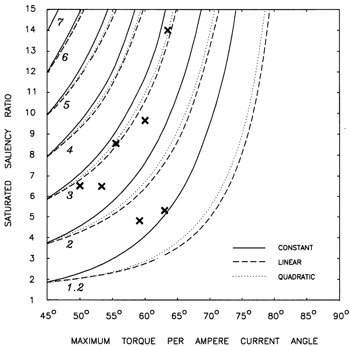
Figure 3.22: Location of practical SYNCHREL designs on CPSR contour plot.
