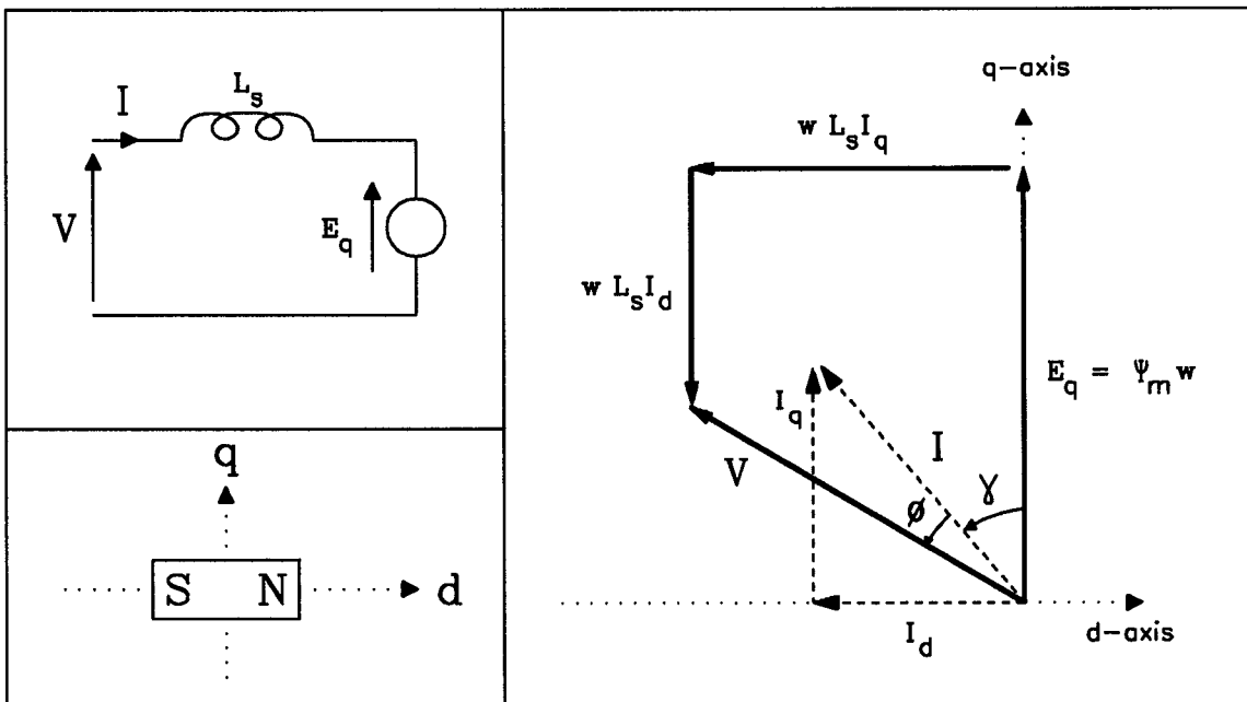
Figure 2.2: Surface permanent magnet motor phasor diagram.
