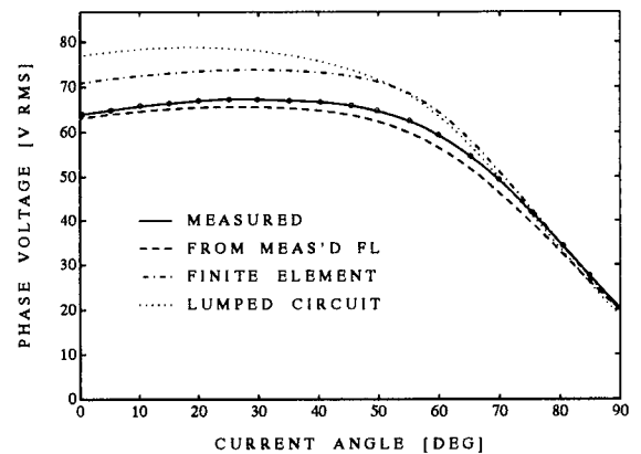
Figure 8: Fundamental phase voltage versus current angle.
