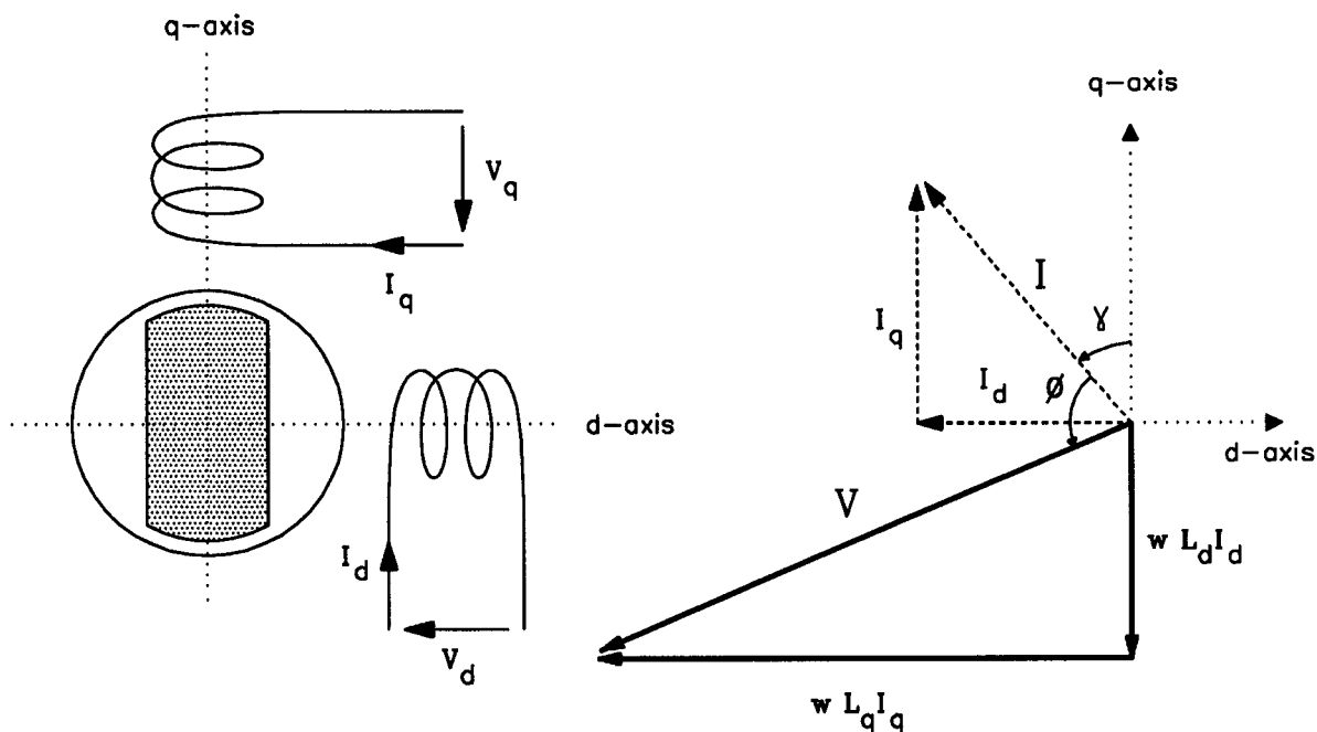
Figure 2.9: Synchronous reluctance motor phasor diagram.
