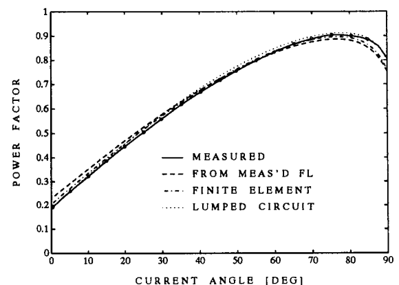
Figure 9: Power-factor versus current angle.
