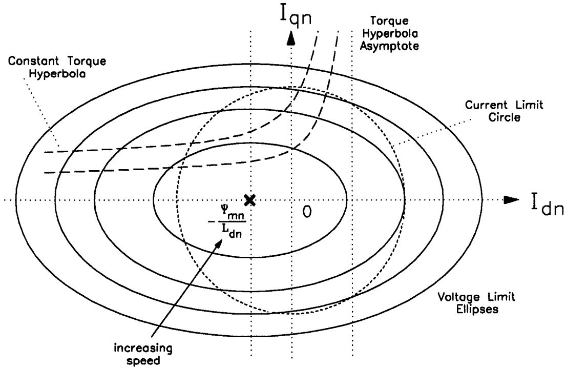
Figure 2.16: The IPM circle diagram.
