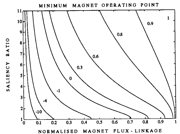
Figure 14: Demagnetisation constraints.
