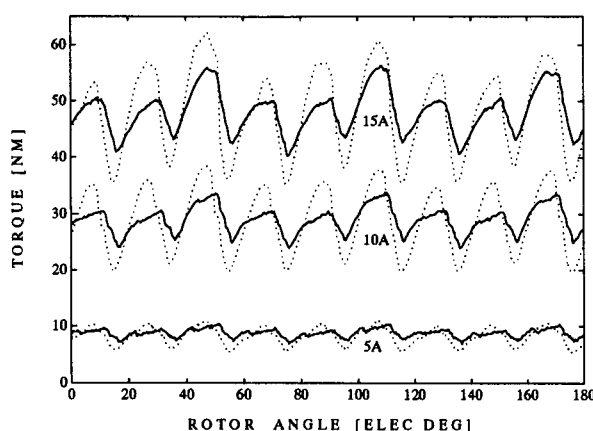
Figure 17: Measured torque ripple for 7.5kW axially-laminated (solid line) and single-barrier (dotted line) synchronous reluctance motor at three levels of current ( \gamma = 45^\circ ).
