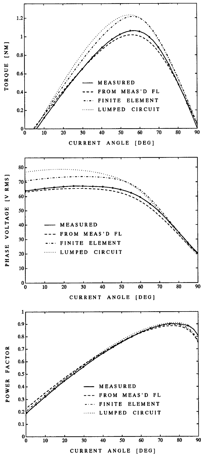
Figure 4.16: Comparison between the 120W calculated and measured characteristics for the torque, voltage and power-factor versus current-angle.
