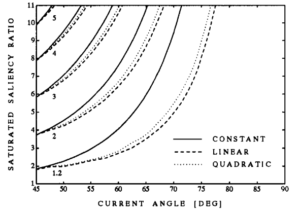
Figure 8: Comparison of the CPSR predicted by the three saturation models for SYNCHRELS.
