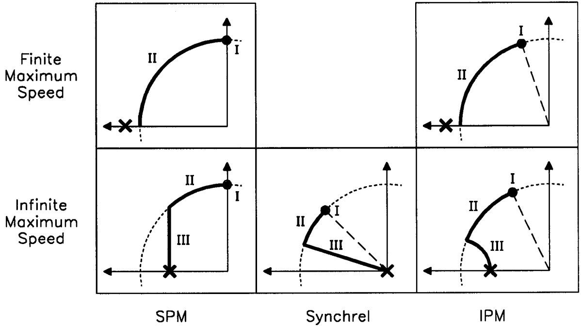
Figure 2.17: The optimal control strategies for the five drive classes.
