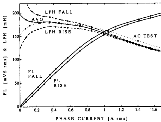
Figure 5: Experimental results from AC and flux-linkage tests.
