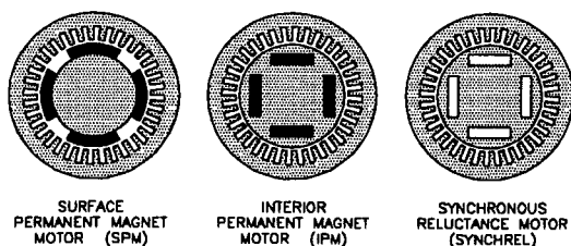
Figure 1: Motor cross-sections.
