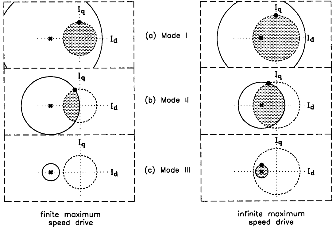
Figure 2.4: Operating modes for finite and infinite maximum speed SPM drives.
