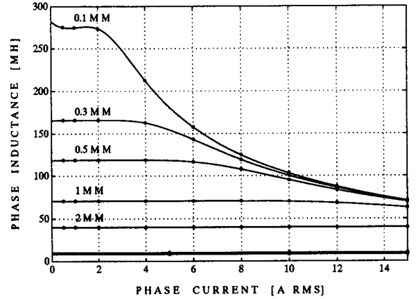
Figure 9: Calculated flux-linkage characteristics for a 7.5kW synchronous reluctance motor with different airgaps.
