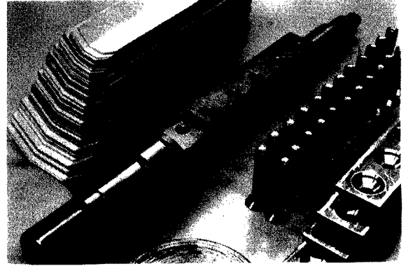
Figure 3: 7.5kW rotor components before assembly.
