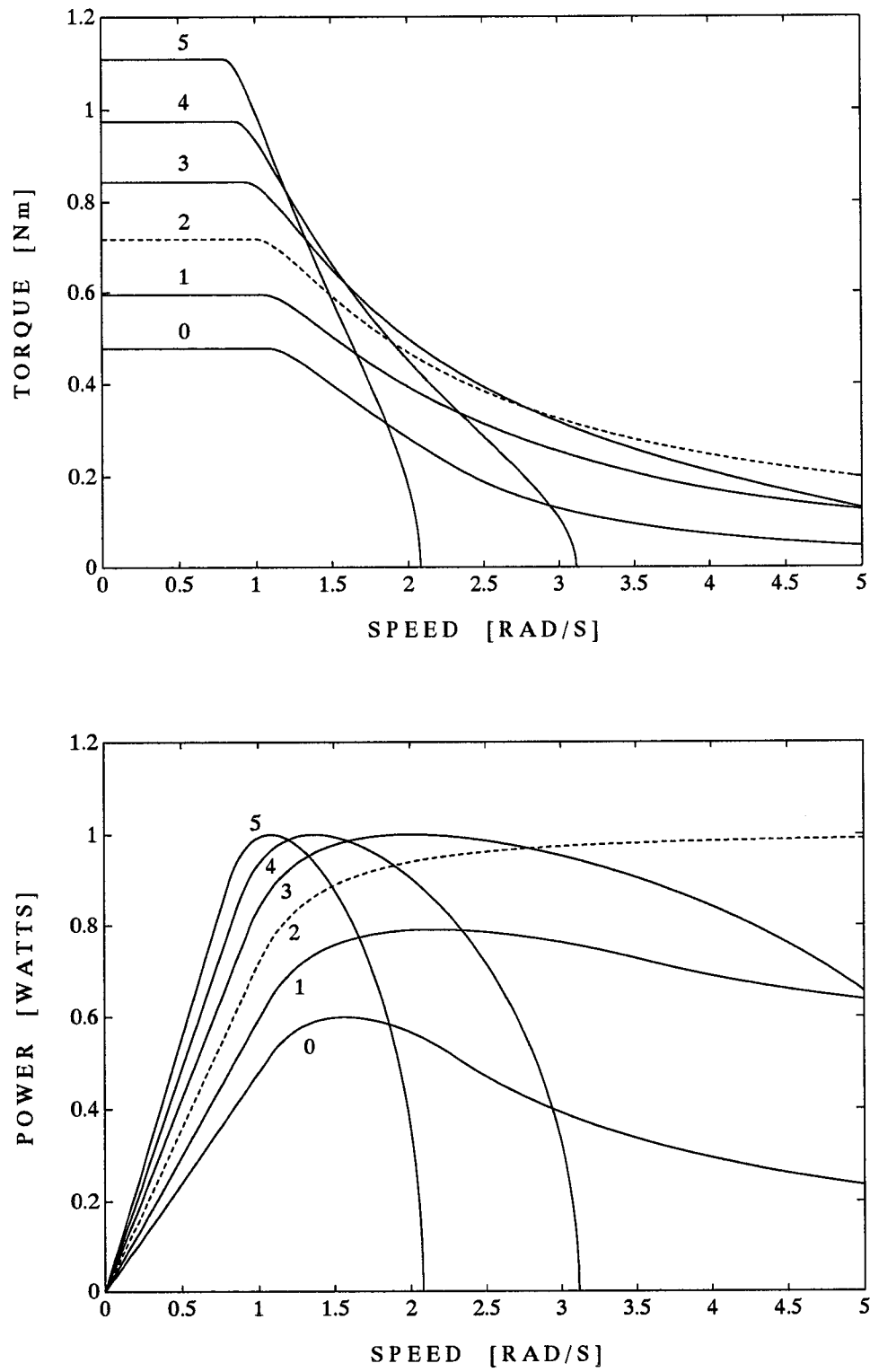
Figure 2.31: Effect of adding magnet material to a SYNCHREL with \xi = 4 .
