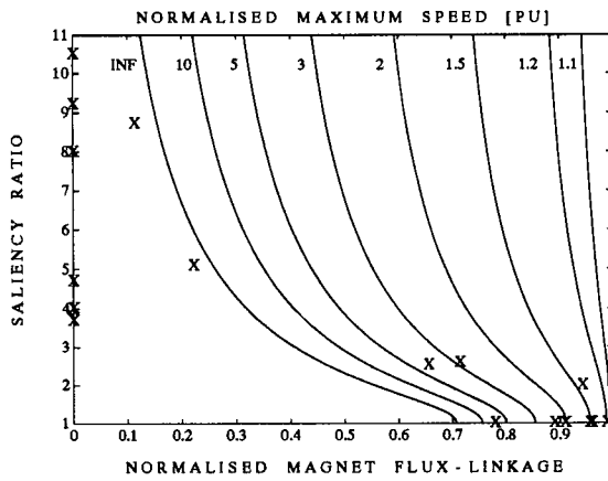
Figure 10: Normalised maximum operating speed ( \omega_{xn} ) and the location of actual drive designs ("x").
