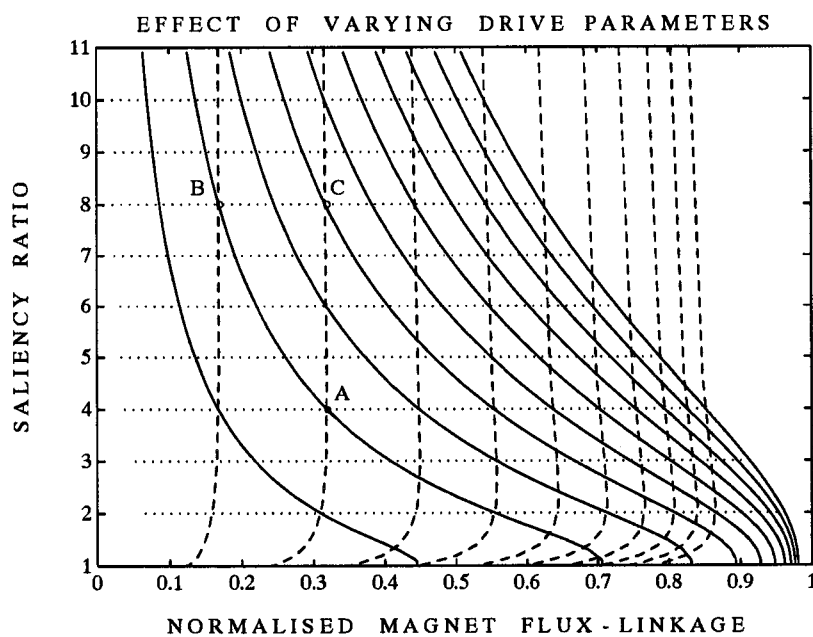
Figure 2.29: Effect of varying L_q (solid), L_d (dashed), \Psi_m and I_o (dotted).
