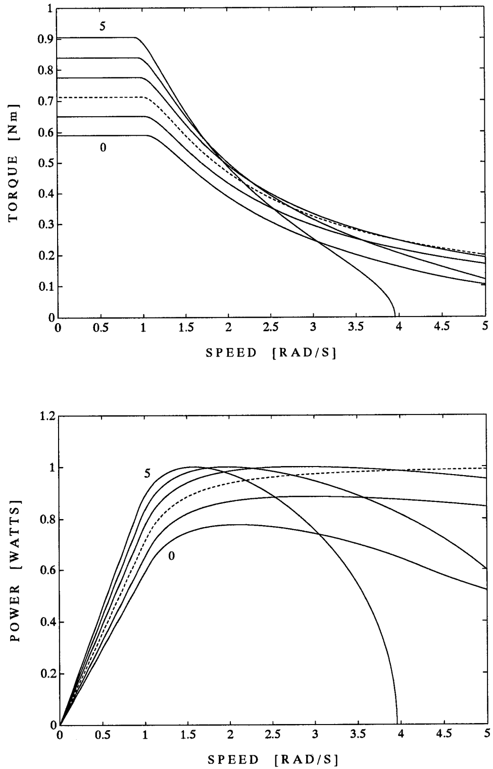
Figure 2.32: Effect of adding magnet material to a SYNCHREL with \xi = 8 .
