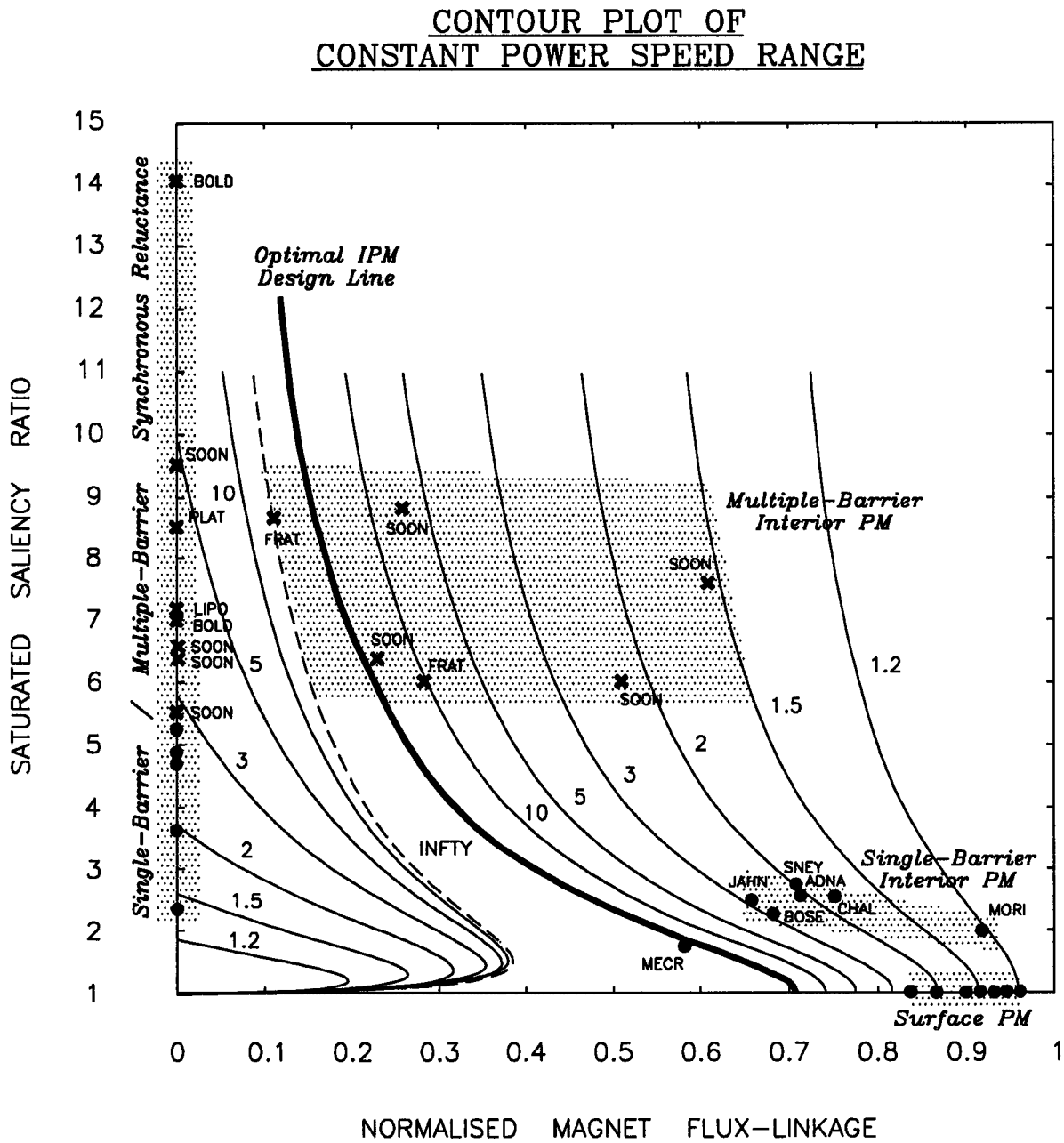
Figure 3.1: Location of motor drive designs in the IPM parameter plane.
