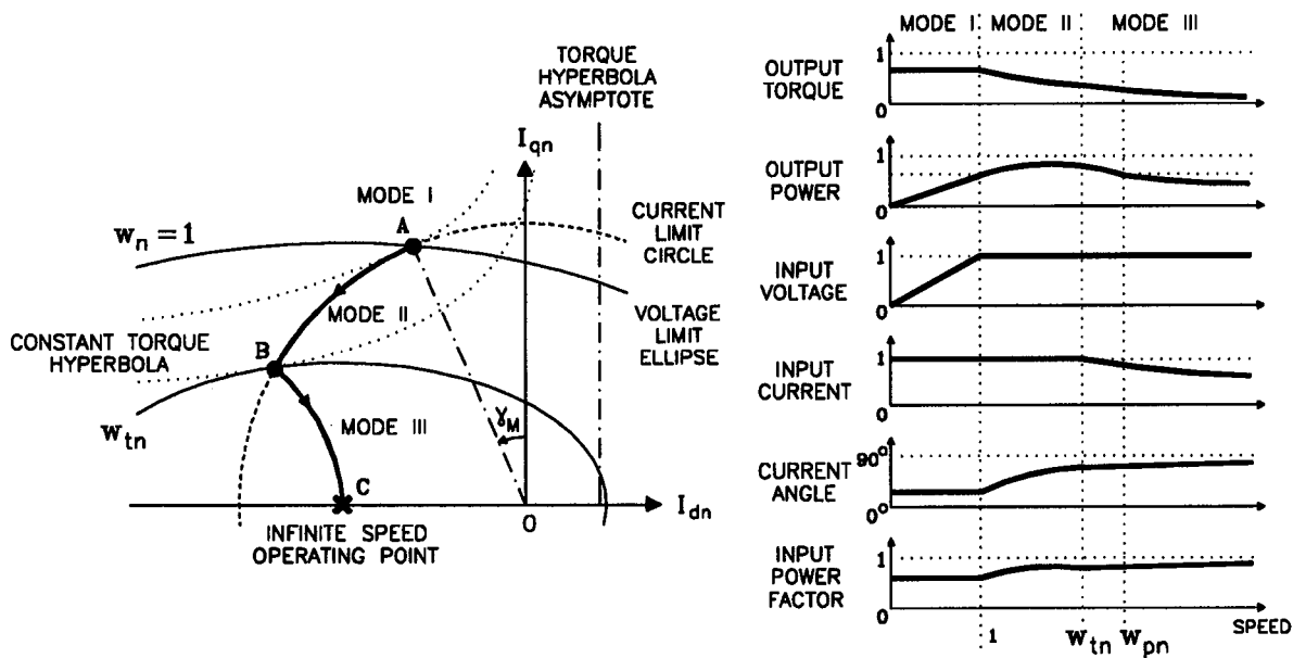
Figure 2.19: The infinite maximum speed IPM operating trajectory.
