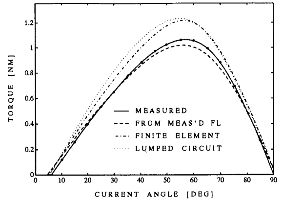
Figure 7: Torque versus current angle.
