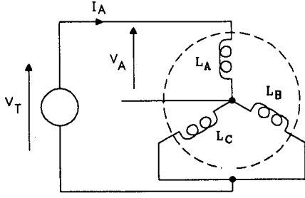
Figure 1: Test circuit for measurement and calculation of the synchronous phase inductance.
