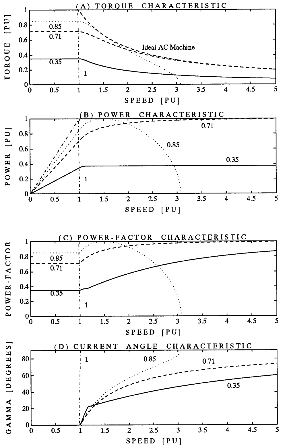
Figure 2.8: Calculated SPM characteristics with \Psi_{mn} as a parameter.
