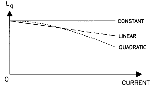
Figure 7: Three saturation models.
