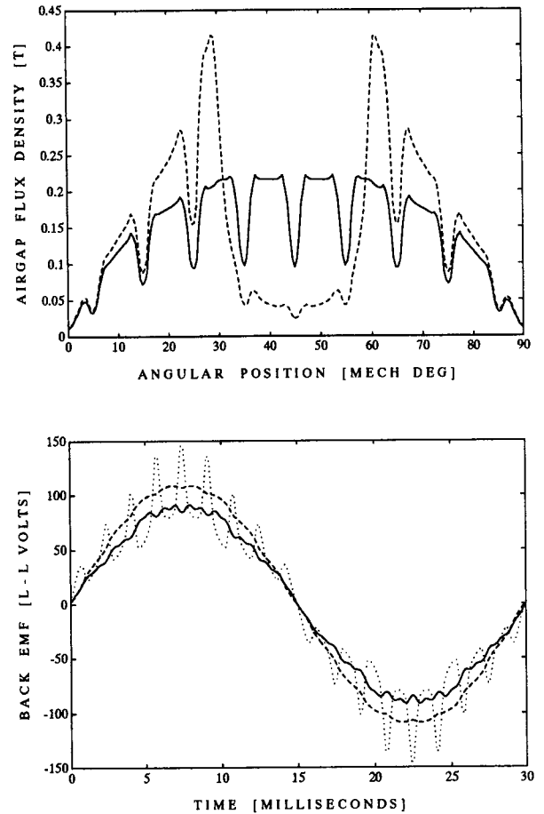
Figure 13: Calculated airgap flux distribution (top) with magnetic (solid line) and non-magnetic (dashed line) pole-pieces. Back-emf waveforms at 1000rpm (bottom) : calculated with magnetic (dashed line) and non-magnetic (dotted line) pole-pieces and measured waveform with magnetic pole-pieces (solid line).
