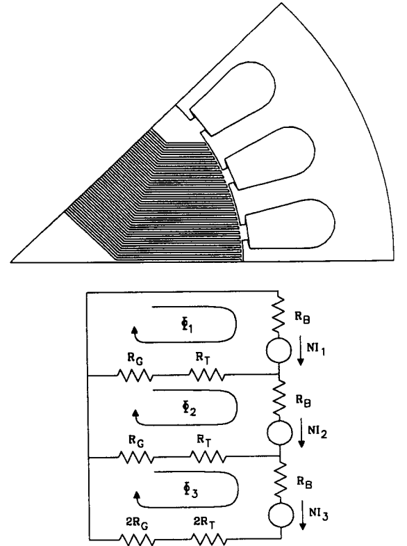
Figure 3: 120W rotor cross-section and lumped-circuit model (q-axis case).
