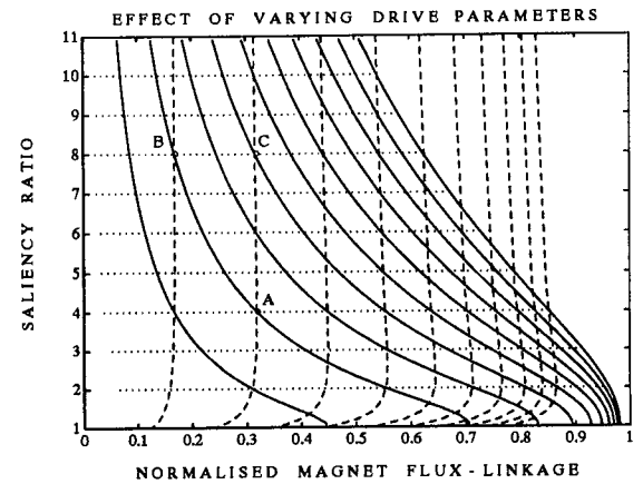
Figure 13: Effect of varying L_q (solid), L_d (dashed), \Psi_m and I_o (dotted).
