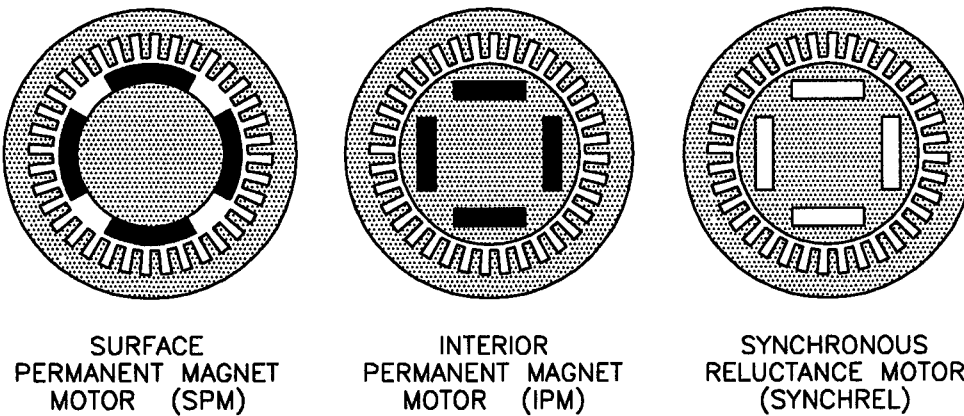
Figure 2.1: Motor cross-sections.
