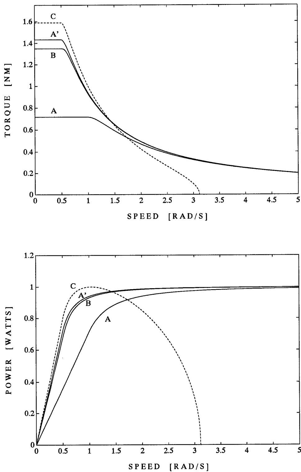
Figure 2.30: Effect of parameter changes on the torque versus speed characteristic.
