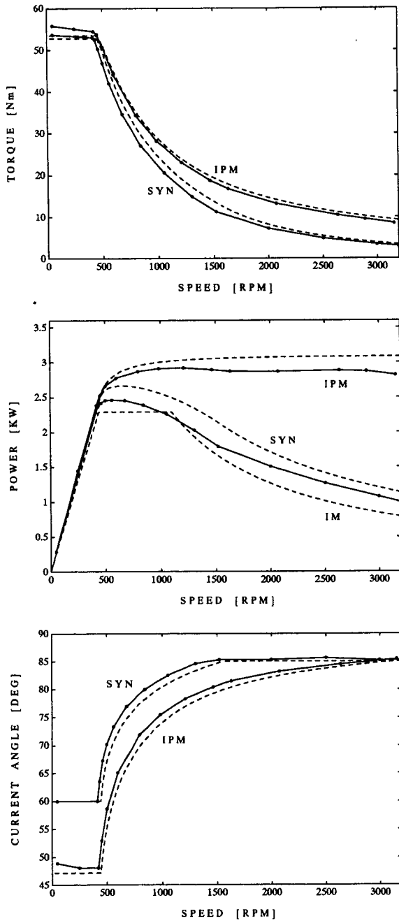
Figure 16: Field-weakening characteristics at rated current and one third of rated voltage. Measured results (solid lines) and calculated results (dashed lines). The calculated characteristic of the induction motor is given for comparison.
