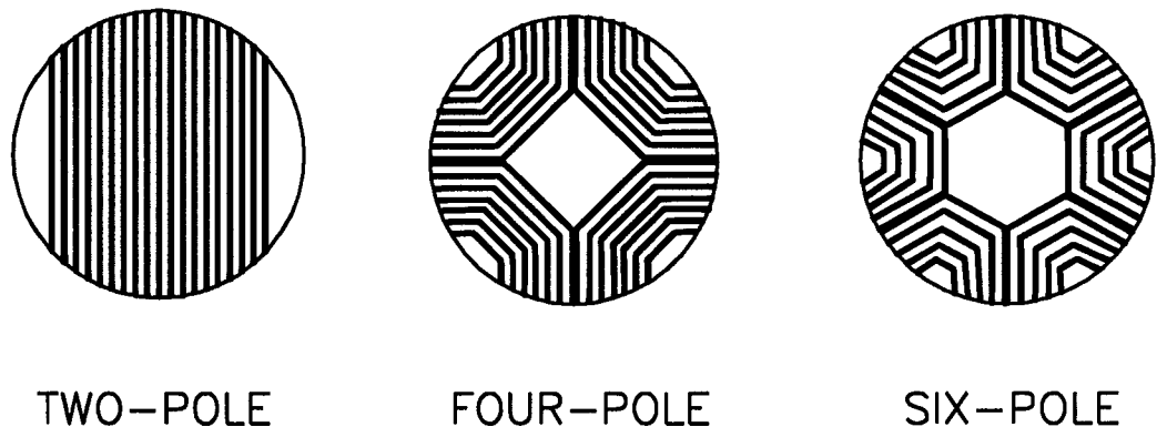
Figure 5.2: Two, four and six-pole rotors
