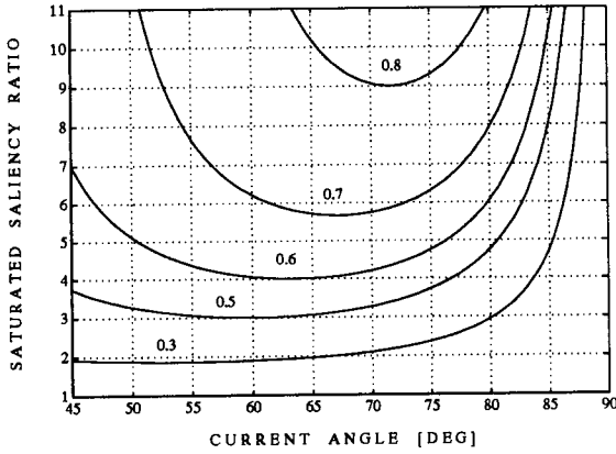
Figure 4: SYNCHREL Mode II inverter utilisation \kappa .
