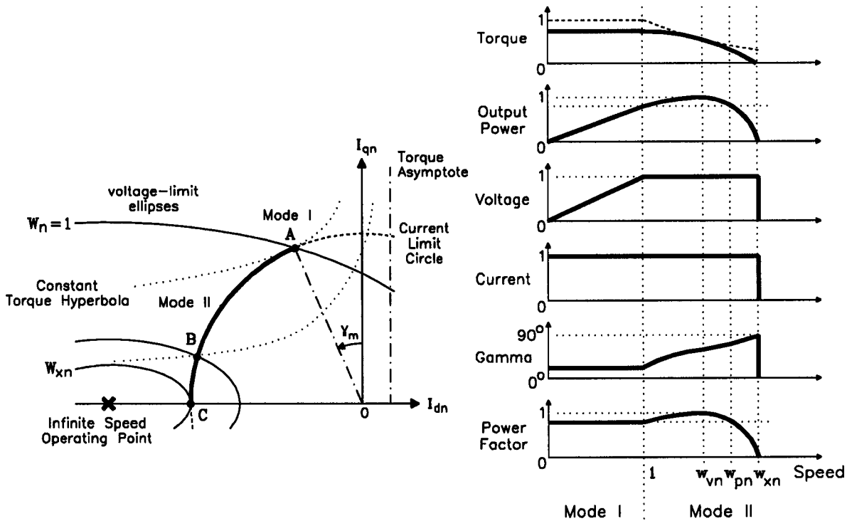
Figure 2.18: The finite maximum speed IPM operating trajectory.
