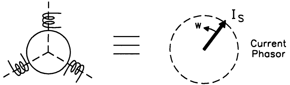
Figure 1.6: The AC stator winding.
