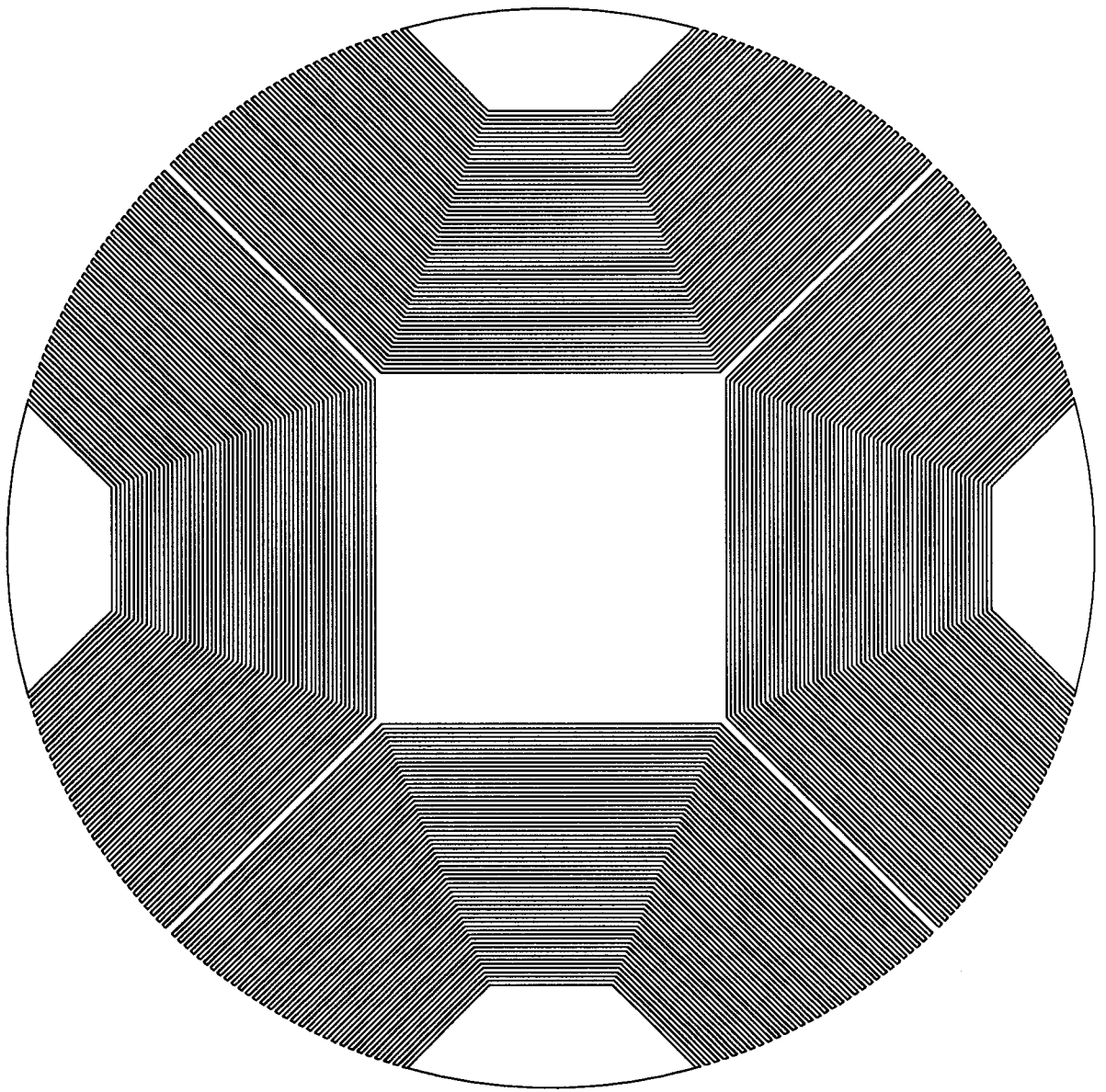
Figure 5.4: 7.5kW axially-laminated rotor cross-sectional view.
