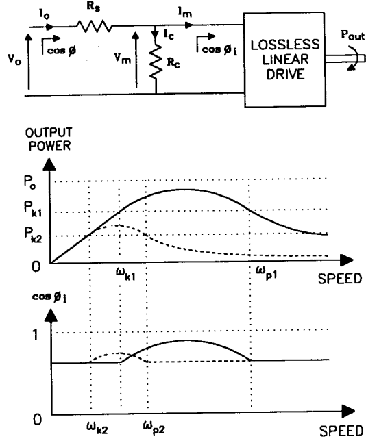
Figure 5: Stator resistance decreases the knee-speed but does not alter the CPSR.
