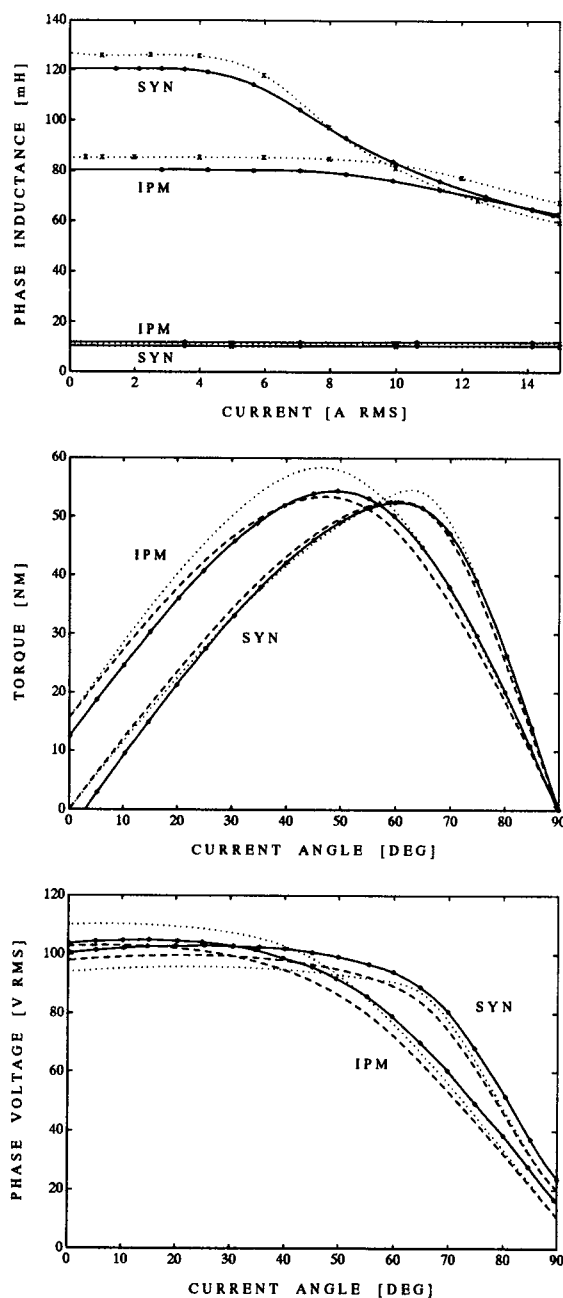
Figure 15: Inductance, torque and fundamental voltage characteristics of the 7.5kW synchronous reluctance (SYN) and interior permanent magnet motor (IPM). The torque and voltage characteristics are measured at 500rpm and 15A. Measured (solid), calculated from the measured inductance characteristics (dashed) and finite-element predictions (dotted).
