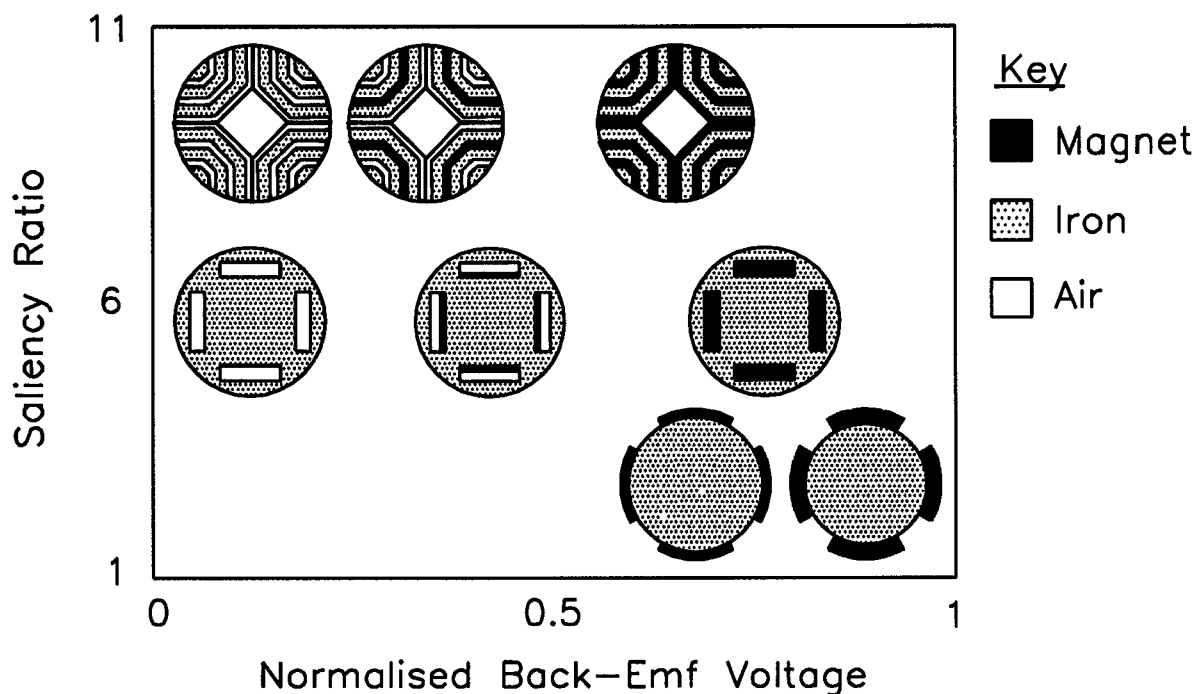
Figure 2.20: The IPM parameter plane.
