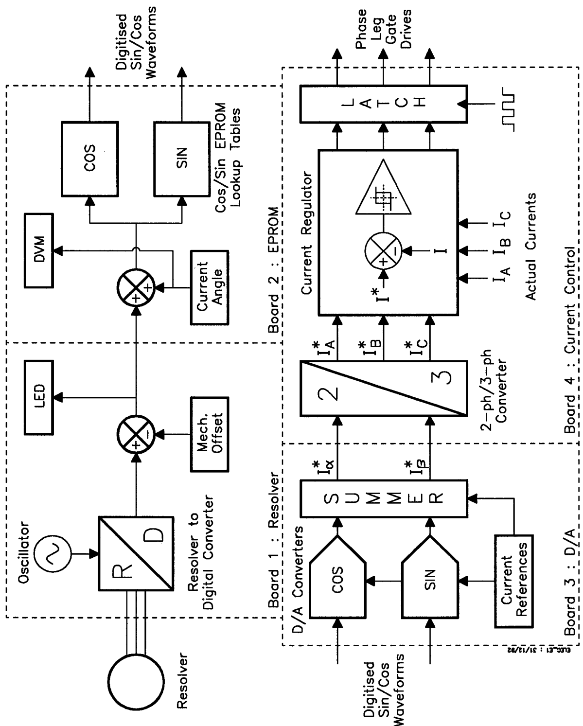
Figure A.3: Block diagram of analog current controller.
