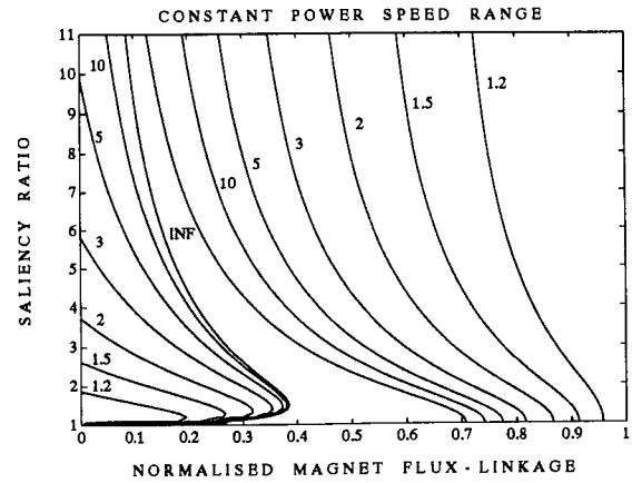
Figure 12: Constant power speed range (CPSR).
